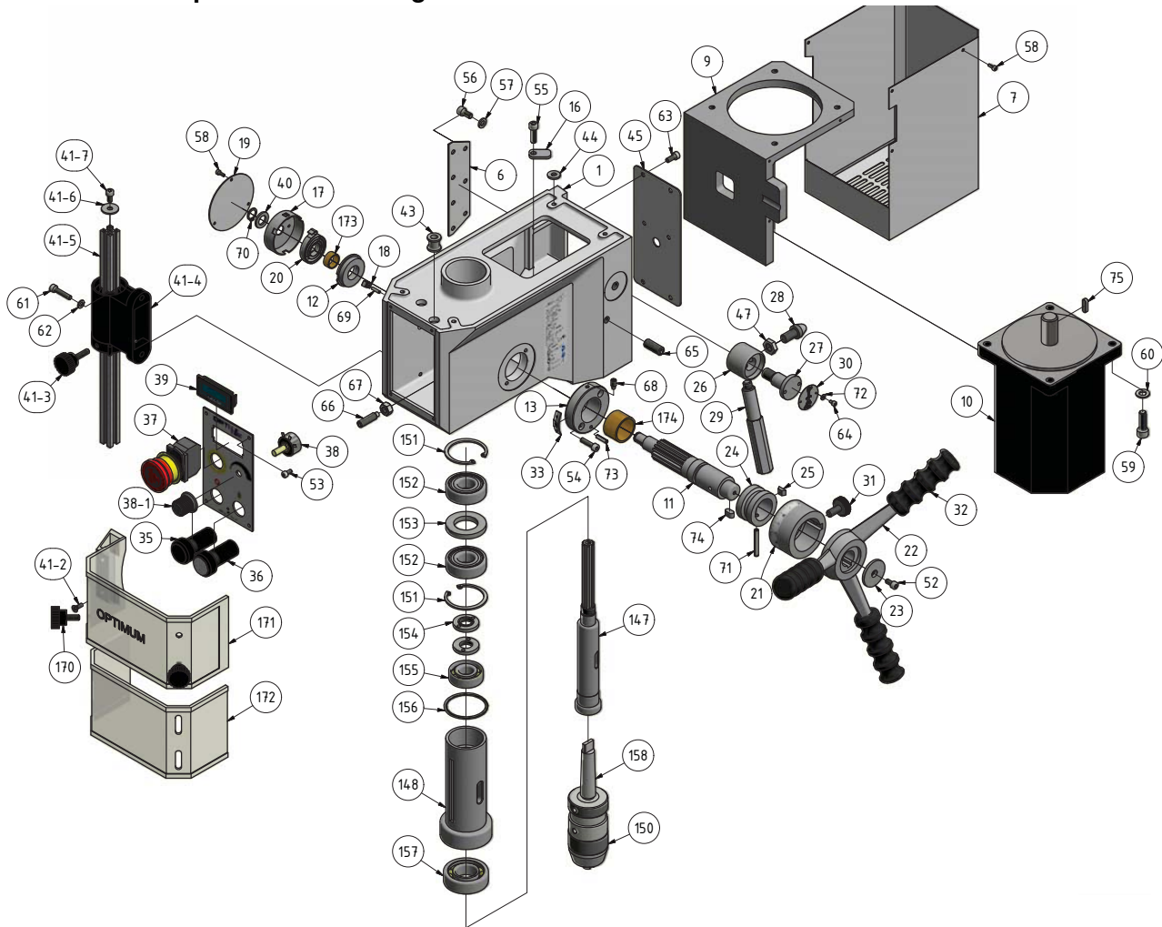
Abb.1-4: Bohrkopf - Drilling head
