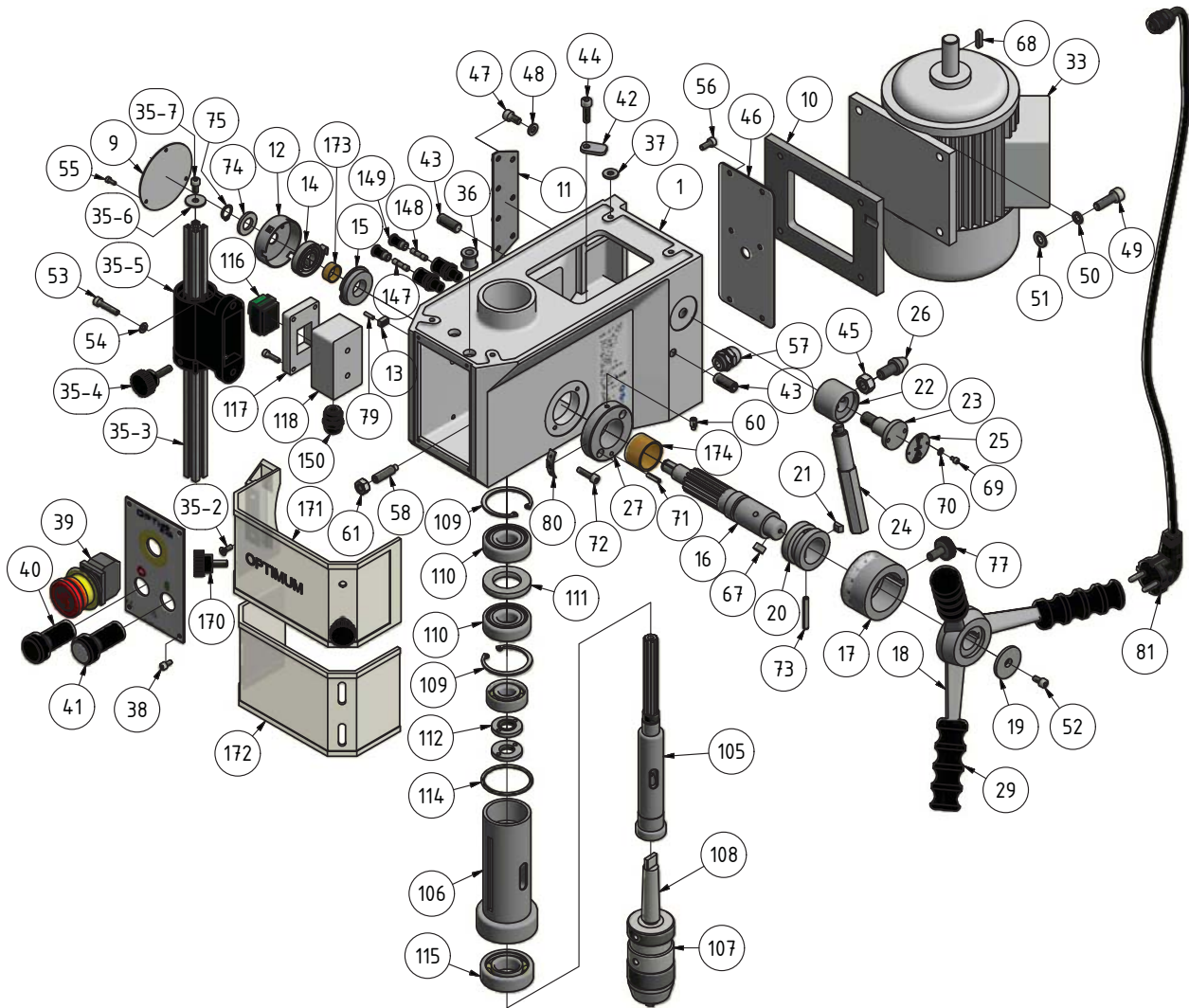
Abb.1-1: Bohrkopf B16H - Drilling head B16H
